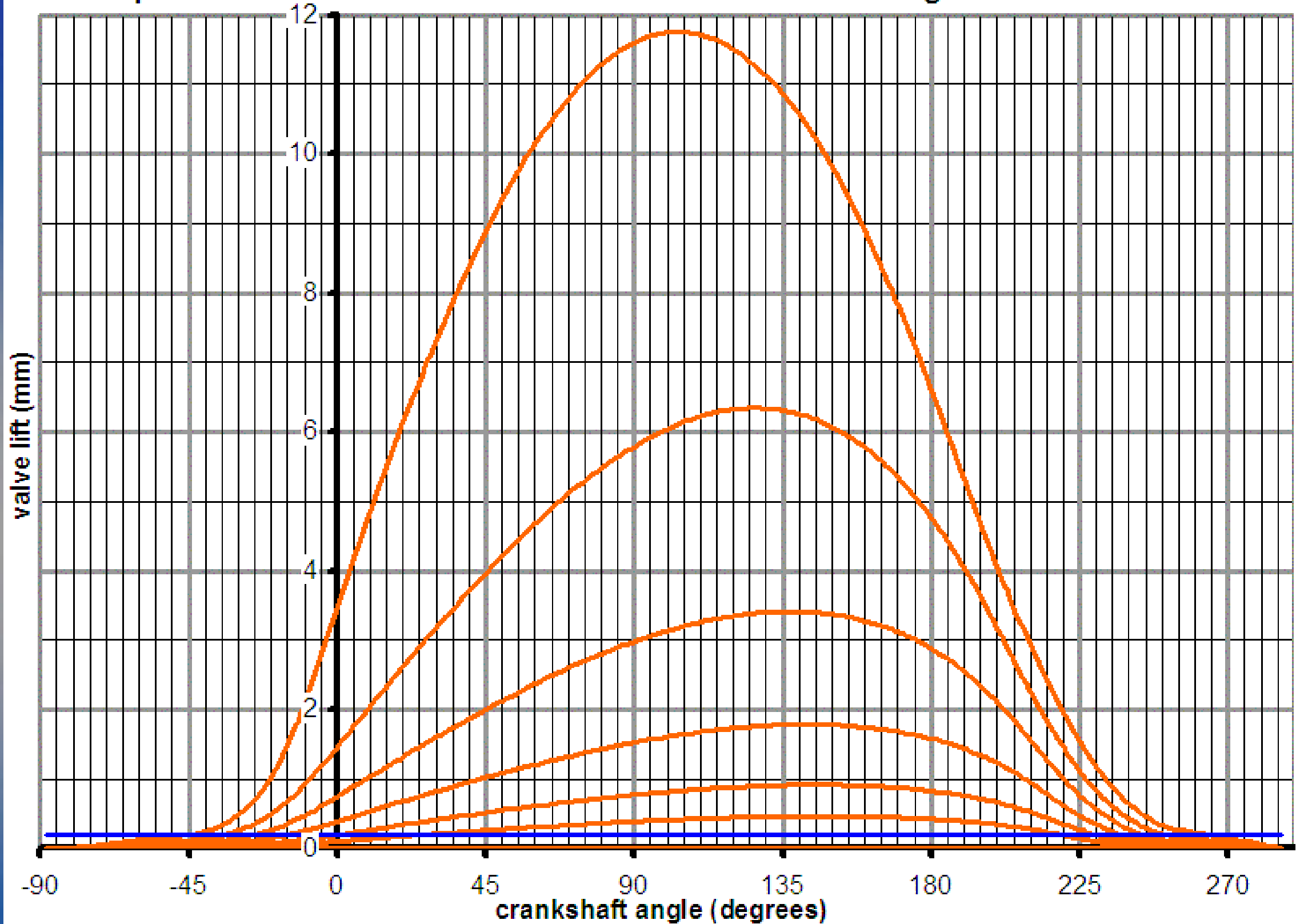
pattakon "rod-roller" VVA at intake side of Citroen-Peugeot 1600cc / 16v
