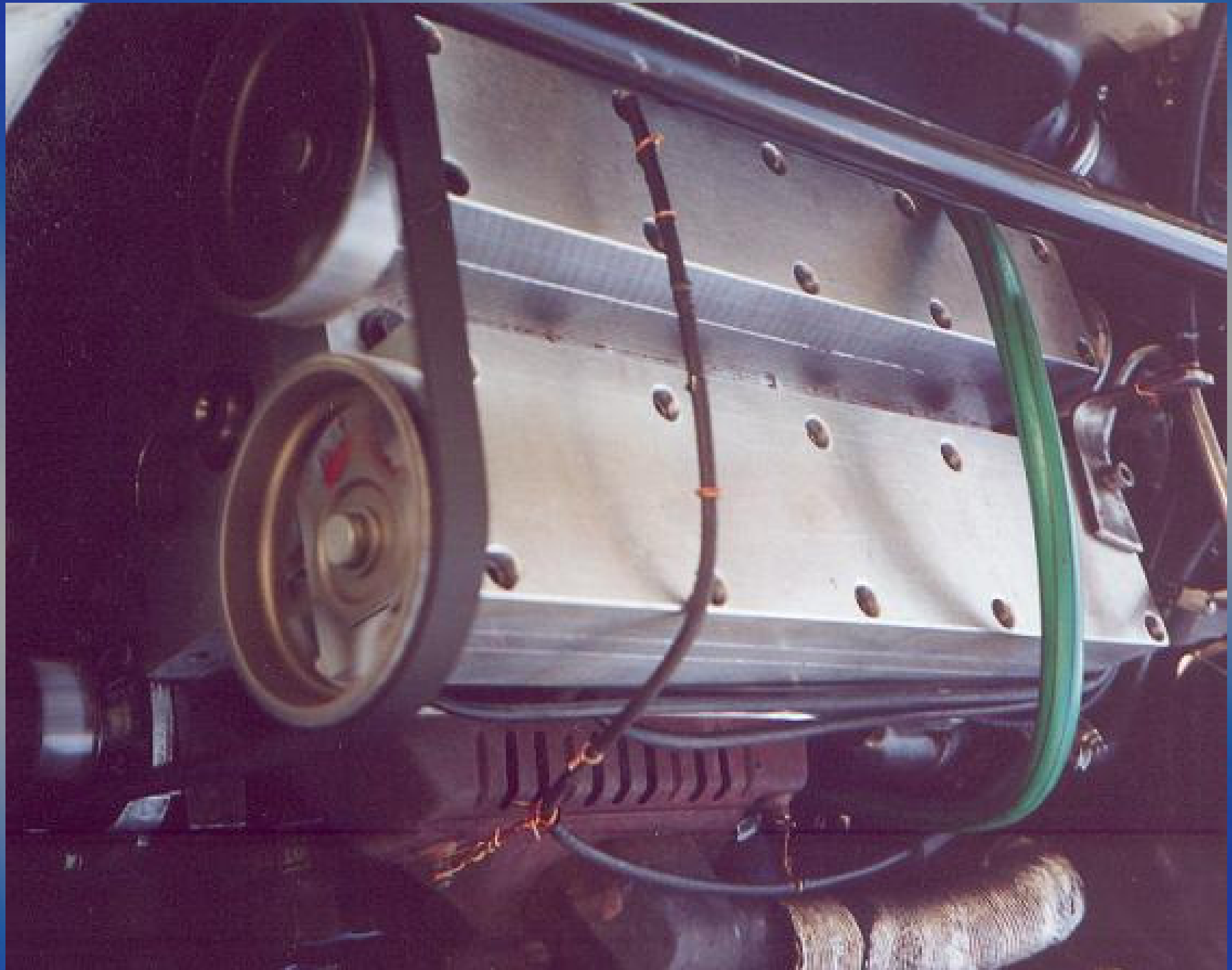
The cylinder head of the 1 st pattakon prototype VVA
